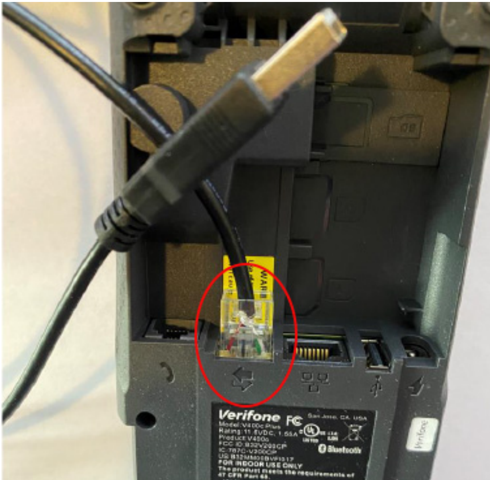
Figure 1 - USB to RJ50 cable connected to the V400c.
