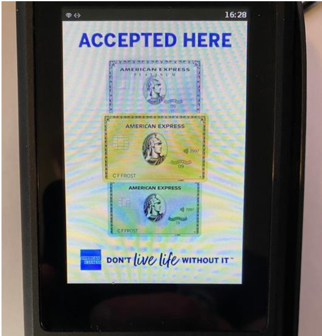
Figure 4 - acceptance screen
